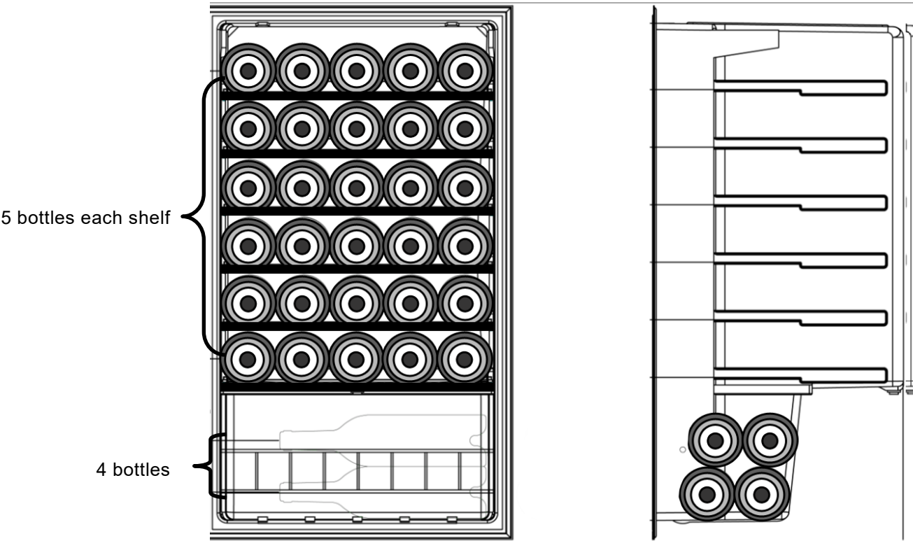
34 BOTTLES LOADING PLAN (6 wooden shelves, wire gate installed)
